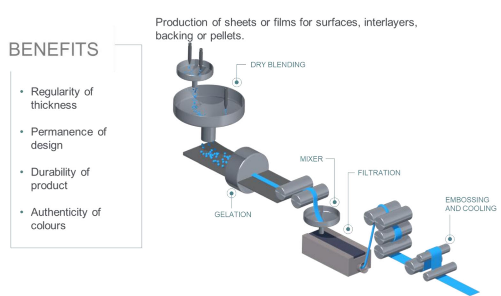
Figure 9: Calendering process
